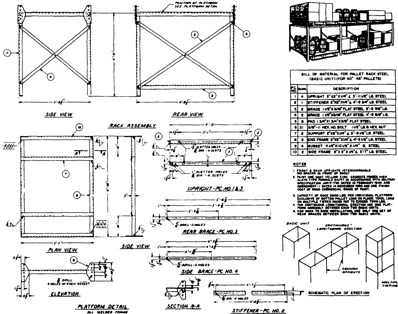
Figure 2-37. Metal Pallet Rack for Storage of Small Lot Items
