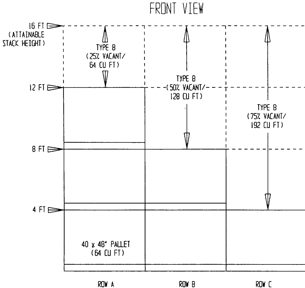
Figure 2-58. Computing Type B Potential Vacant Space
