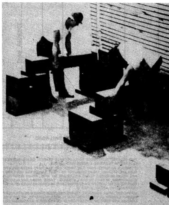
Figure 5-10. Application of the portable lumber foundation.
