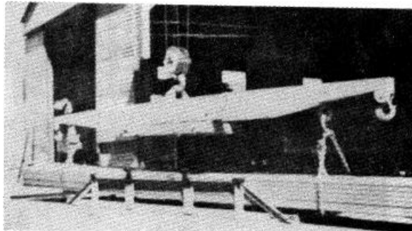
Figure 5-58. Combination crane, automatic grab hook, spreader bar, and nesting rack.
