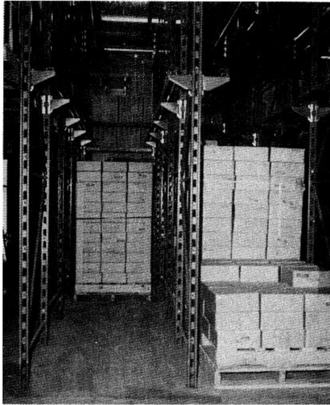
Figure 4-91. Rack, drive-in, drive-through.
