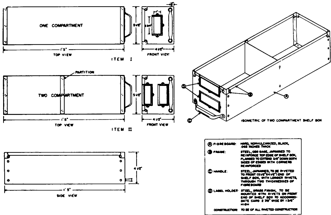
Figure 2-33. Shelf Box, Small, One and Two Compartment
