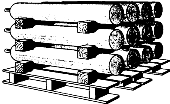
Figure 4-79. Notched spacers.
