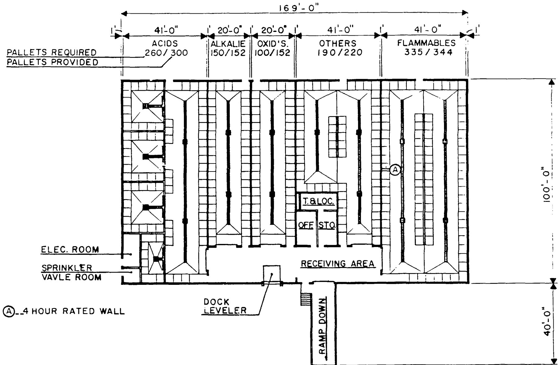
Figure 2-7. Floor Plan of a Flammable/Hazardous Materials Facility
