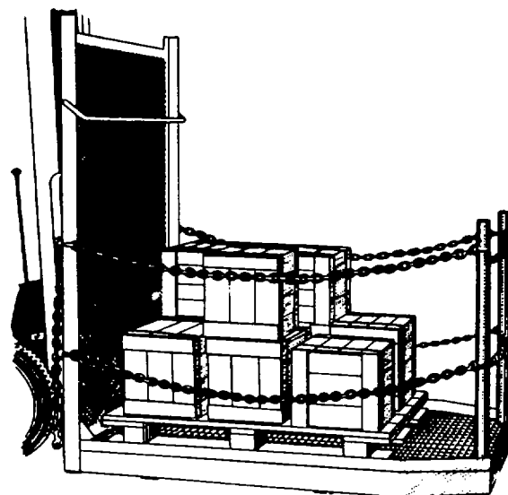
Figure 4-58. Safety pallet
