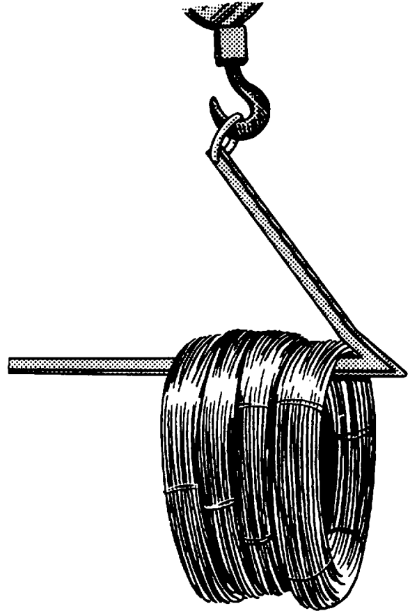
Figure 4-52. Lifting arm bar.
