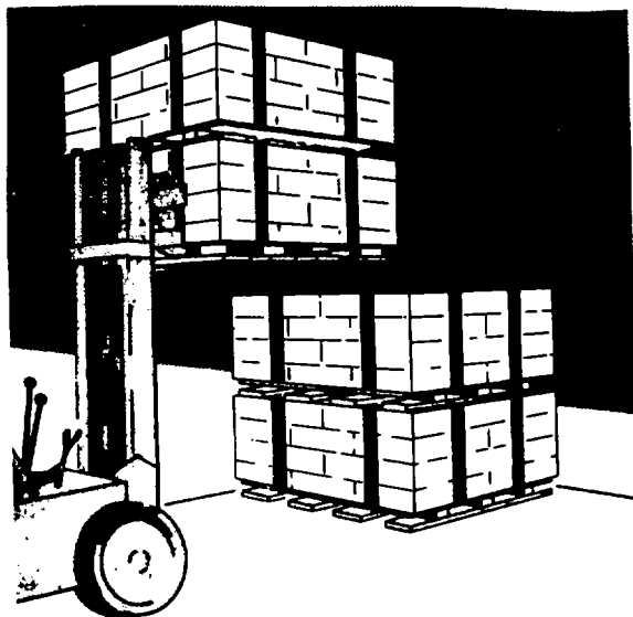
Figure 4-119. A double pallet load must be tied with an overhang of no more than 2 inches in any direction.
