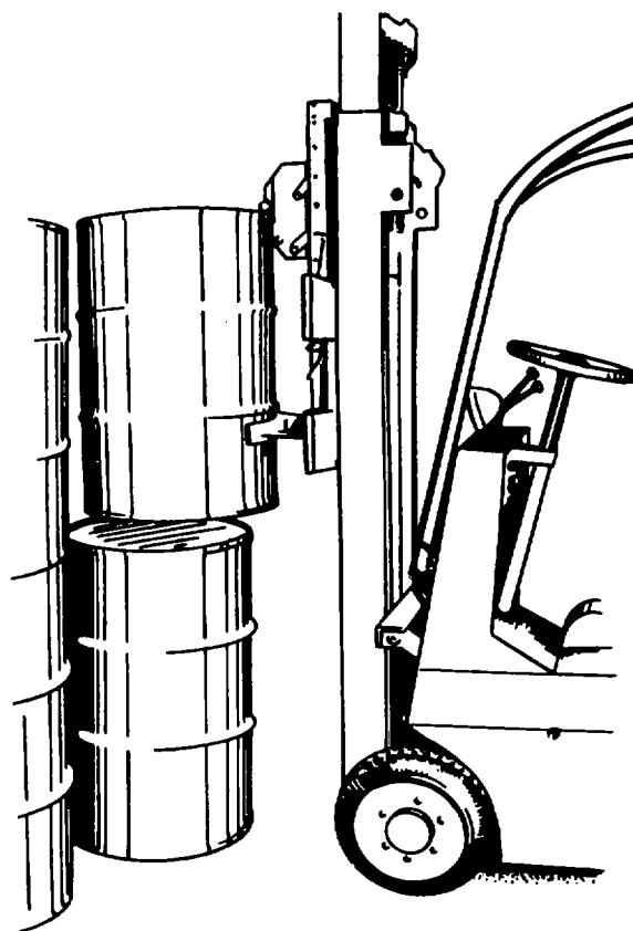
Figure 4-48. Drum-handling attachment single-drum type, vertical carry,
