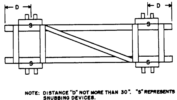
Figure 3-17. Location of snubbing devices.
