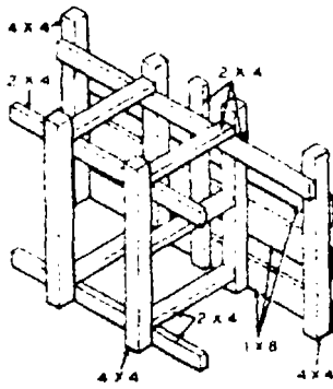
Figure 3-35. Front bulkhead-positioned in trailer, detail of bulkhead.
