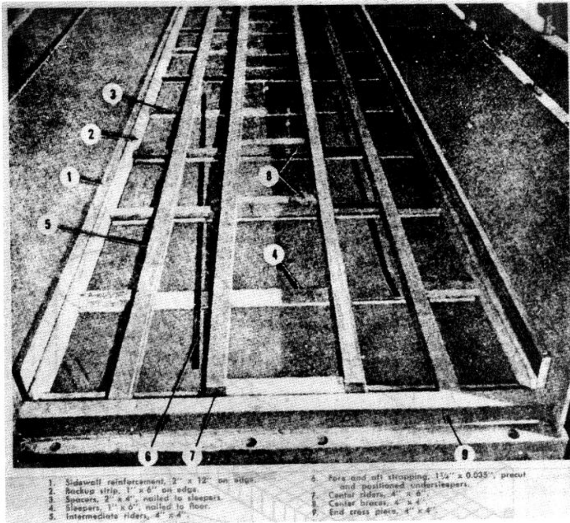
Figure 3-39. Preparatory shoring for cylindrical items.
