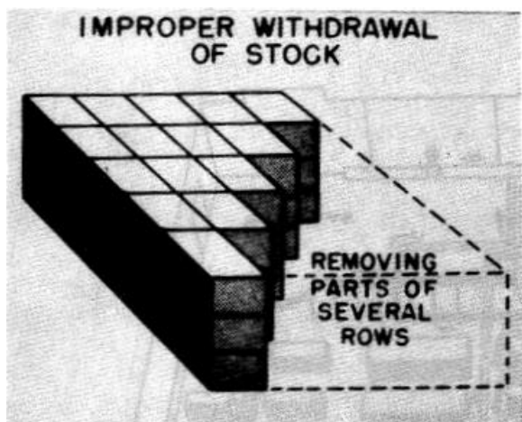
Figure 2-43. Honeycombing Due to Improper Withdrawal of Stock
