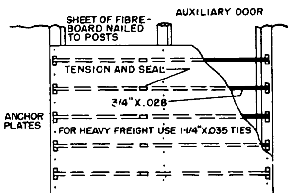
Figure 3-15. Use of steel straps for double door auto boxcar.
