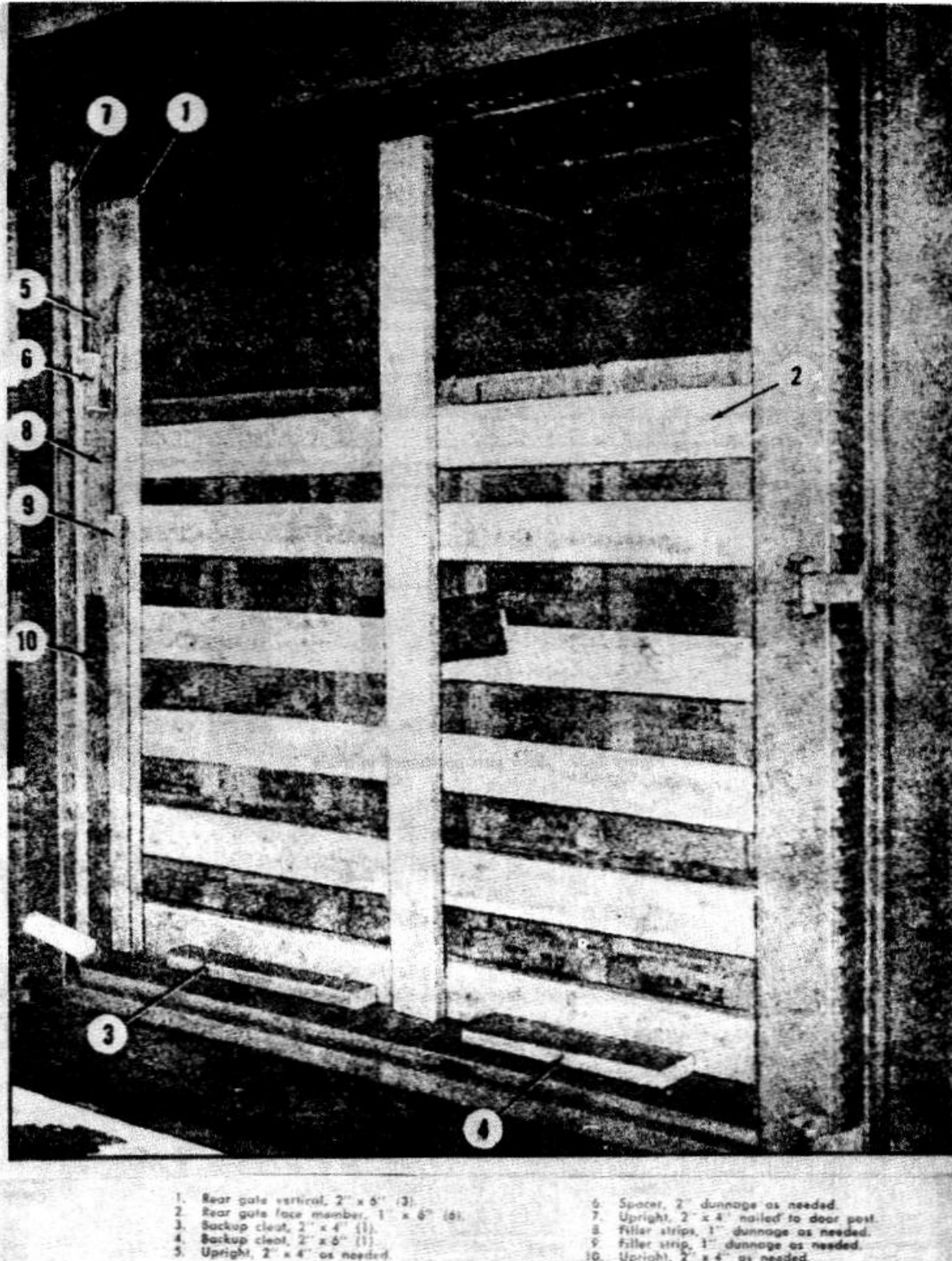
Figure 3-38. Rear gate and dunnage.
