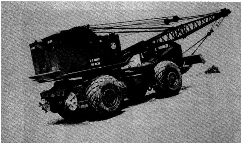
Figure 5-34. Wheel-mounted crane.
