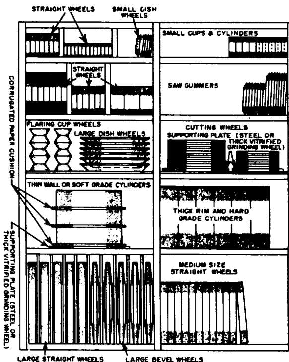
Figure 5-46. Bin storage of grinding wheels.
