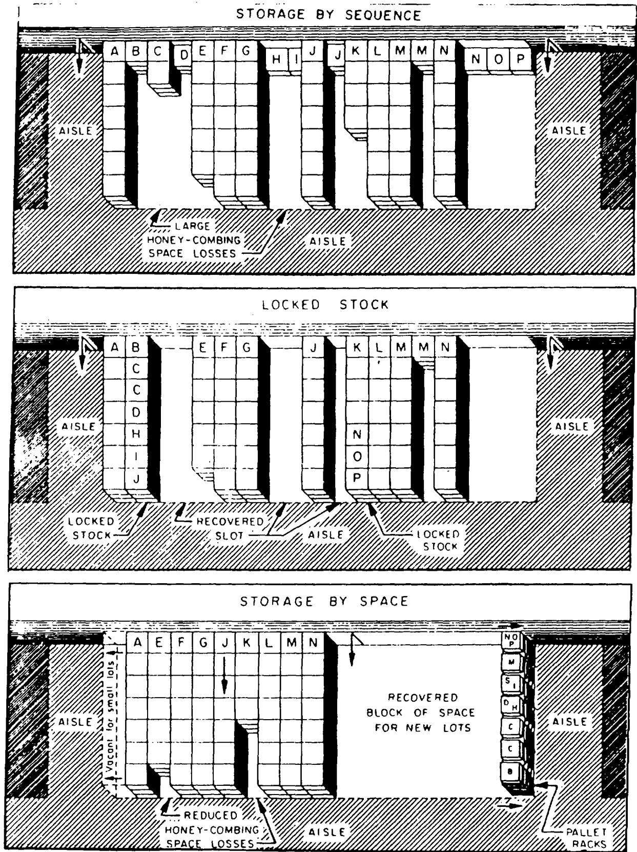
Figure 2-52. Type A Potential Vacant Space Recouped Through Rewarehousing
