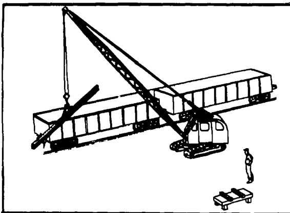
CRANE OPERATION UNLOADING GONDOLA CAR
