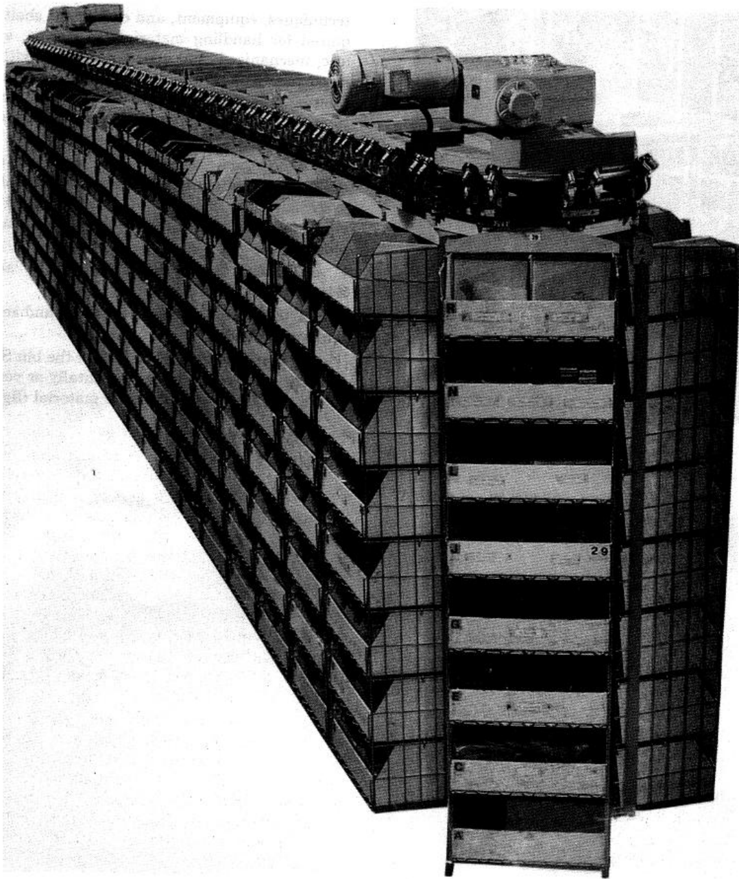
Figure 4-97. Rotary conveyor bins (carousel)
