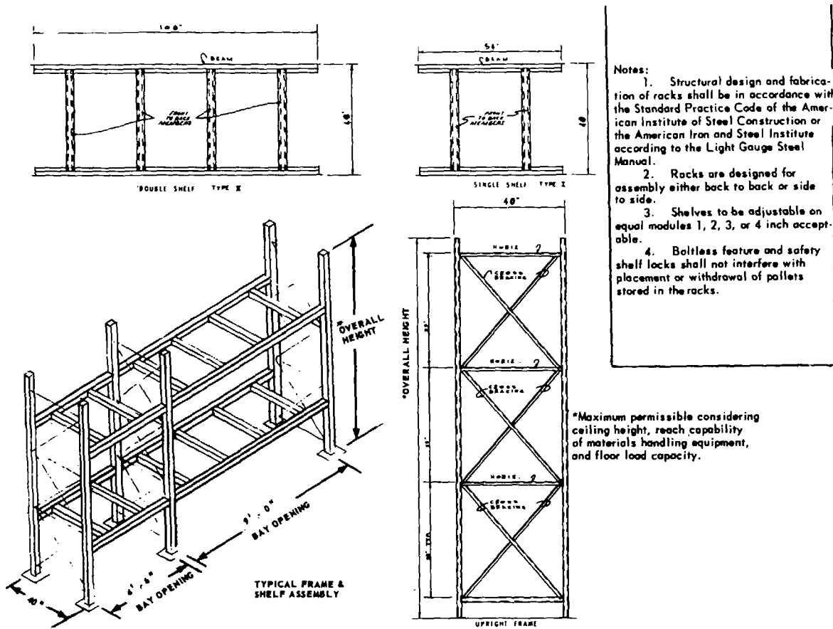
Figure 2-38. Metal Pallet Rack for Storage of Small Lot Items (Boltless Adjustable Type)
