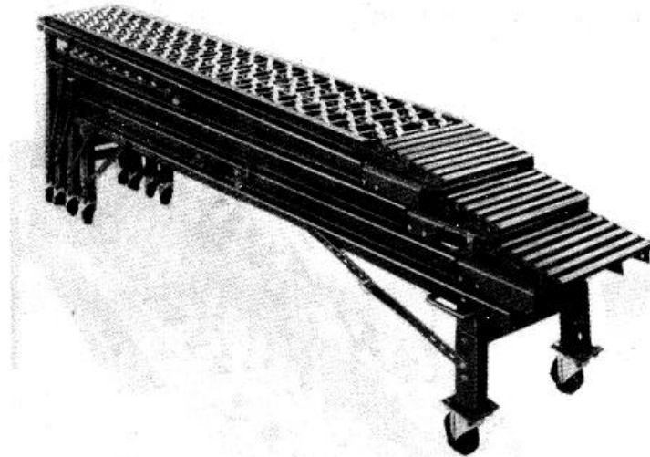
Figure 4-37. Conveyor, gravity extendable
