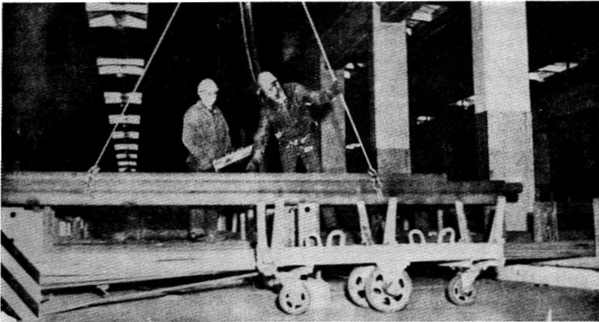
Figure 5-54. Dolly equipped with cradle.
