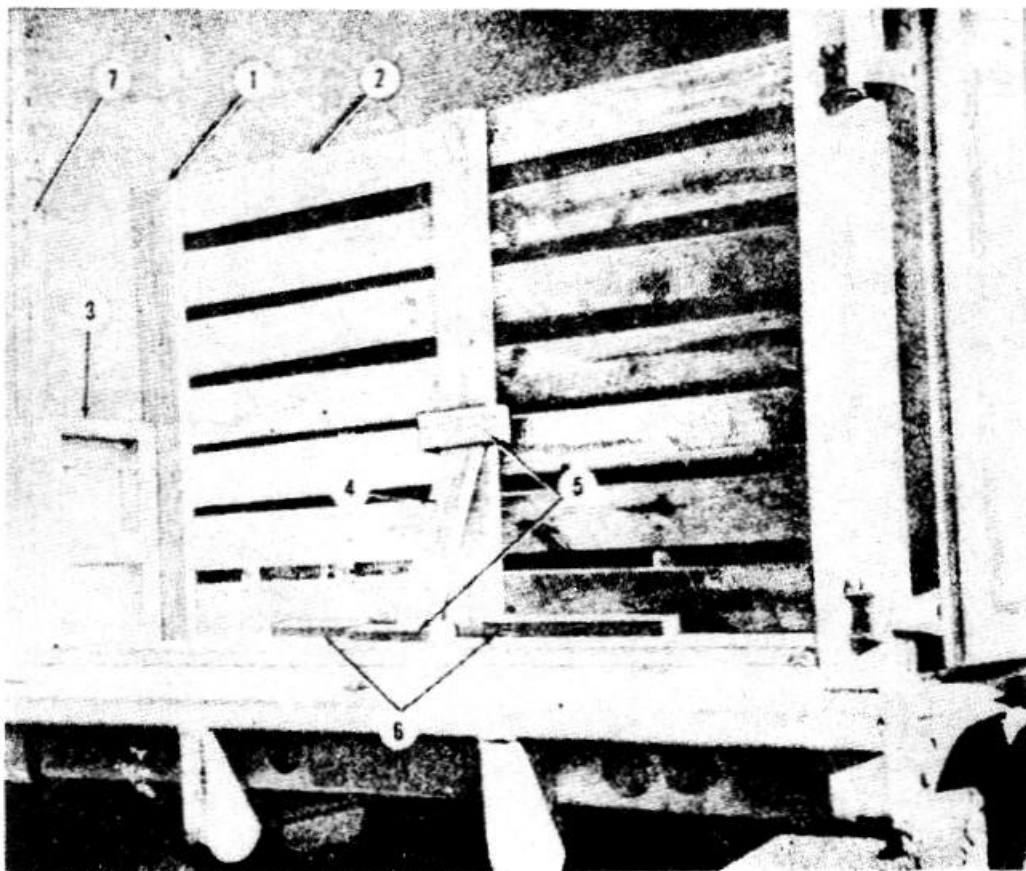
Figure 3-36. Rear gate.
