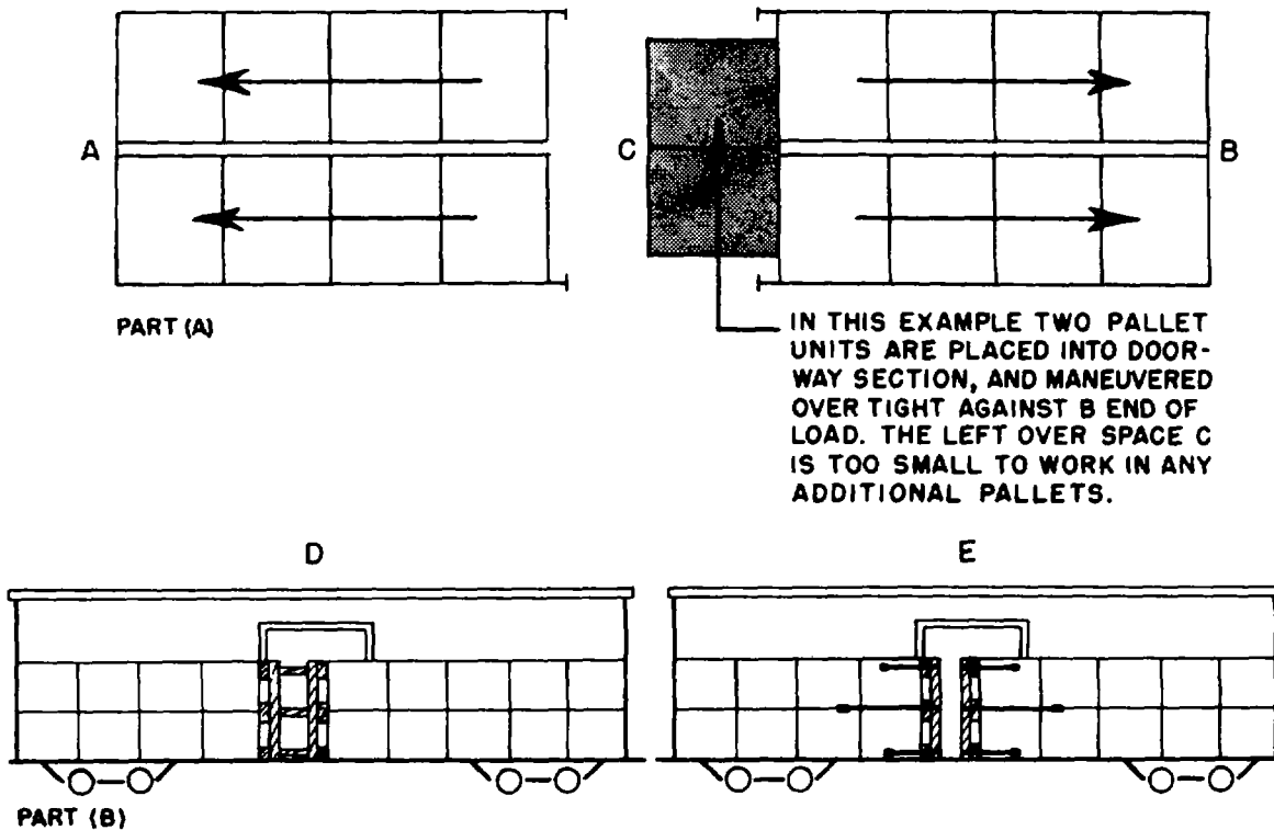
Figure 3-22. Palletized loads.
