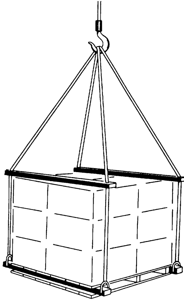
Figure 4-61. Pallet sling.
