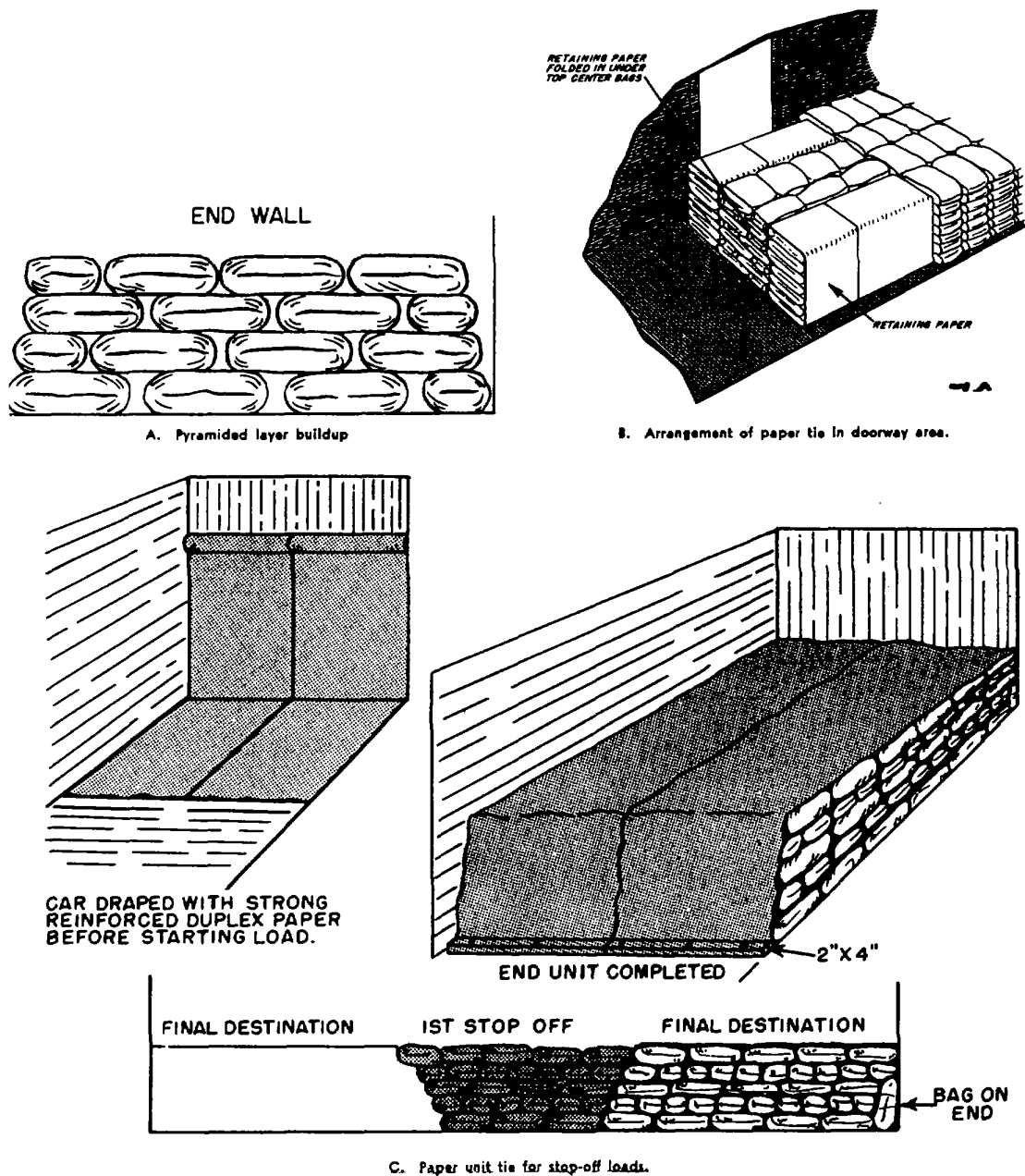
Figure 3-18. Methods to Reduce Chafing
