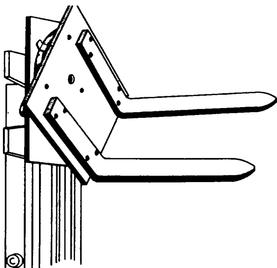
Figure 4-56. Revolving carriage.
