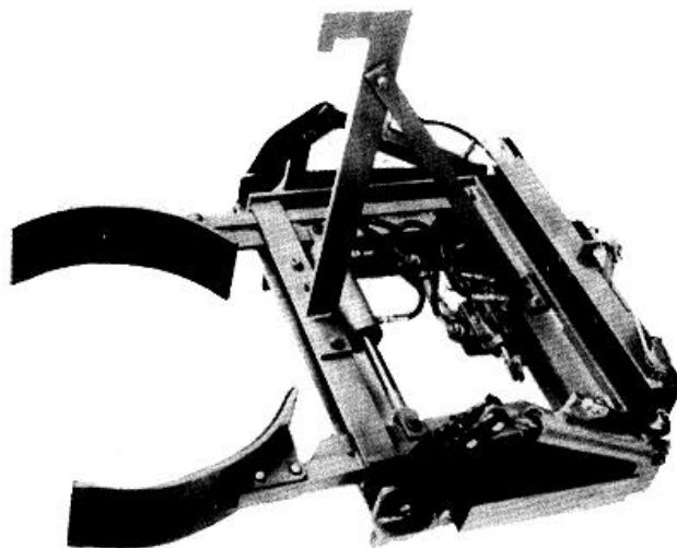
Figure 4-49. Drum-handling adaptor.
