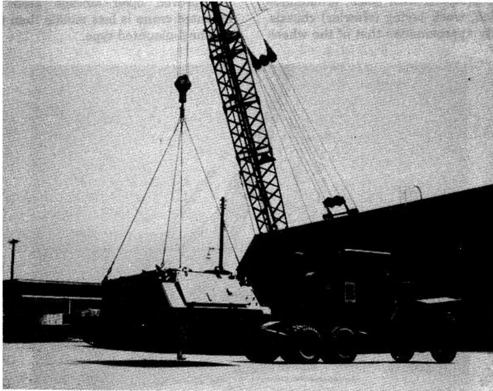
Figure 5-33. Truck-mounted crane.
