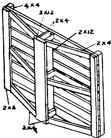
Figure 3-32. Examples of right and wrong truck loading.
