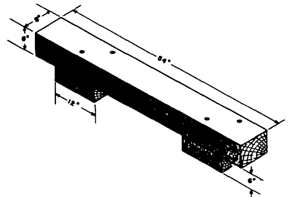
Figure 5-2. Diagram of bolster for use with a 57-inch straddle carry truck.
