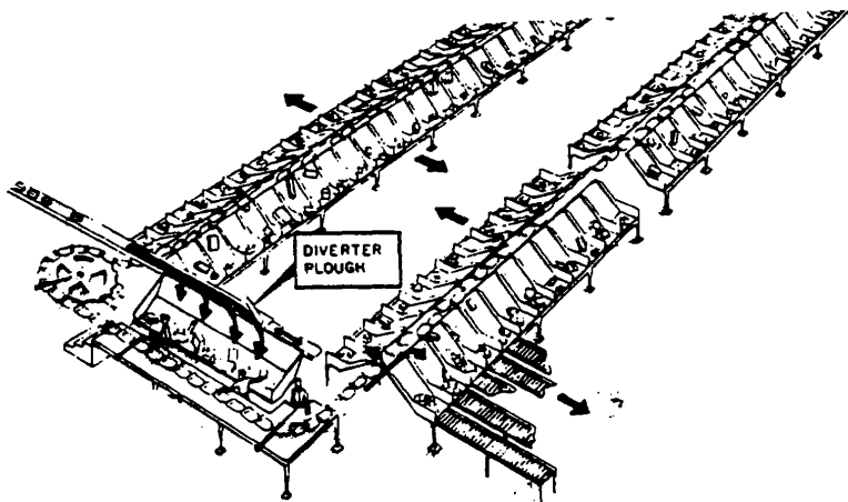
Figure 4-44. Tilt Tray Sorting System.
