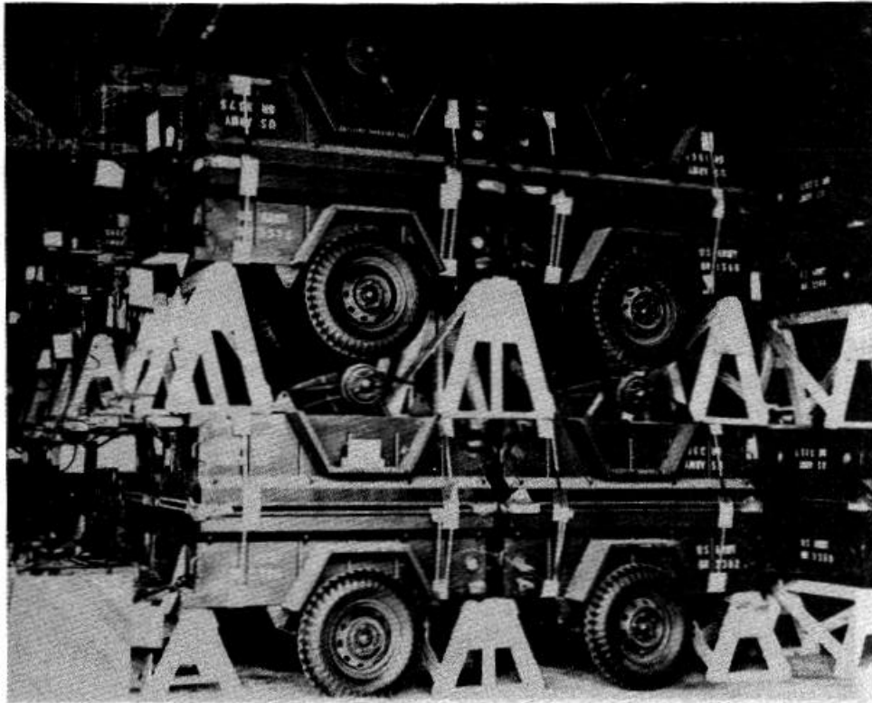
Figure 5-21. Wood stands for stacking vehicles in storage.
