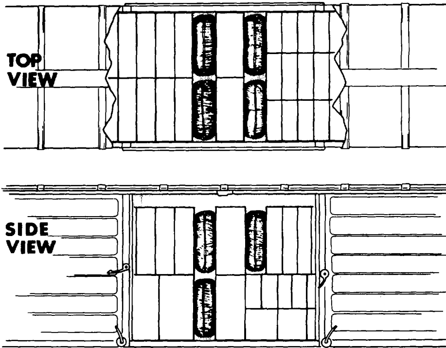
Figure 3-48. Pneumatic dunnage units in various void arrangements.
