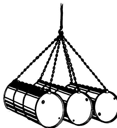
Figure 4-46. Drum-handling sling.
